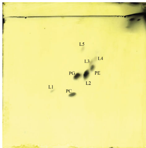
Fig. 2. Two-dimensional thin layer chromatogram of the total polar lipids from strain LHWP3 T , which were detected using 5% ethanolic molybdo-phosphoric acid. Abbreviations: PC, phosphatidylcholine; PG, phosphatidylglycerol; PE, phosphatidylethanolamine; L1–5, unidentified polar lipids.
